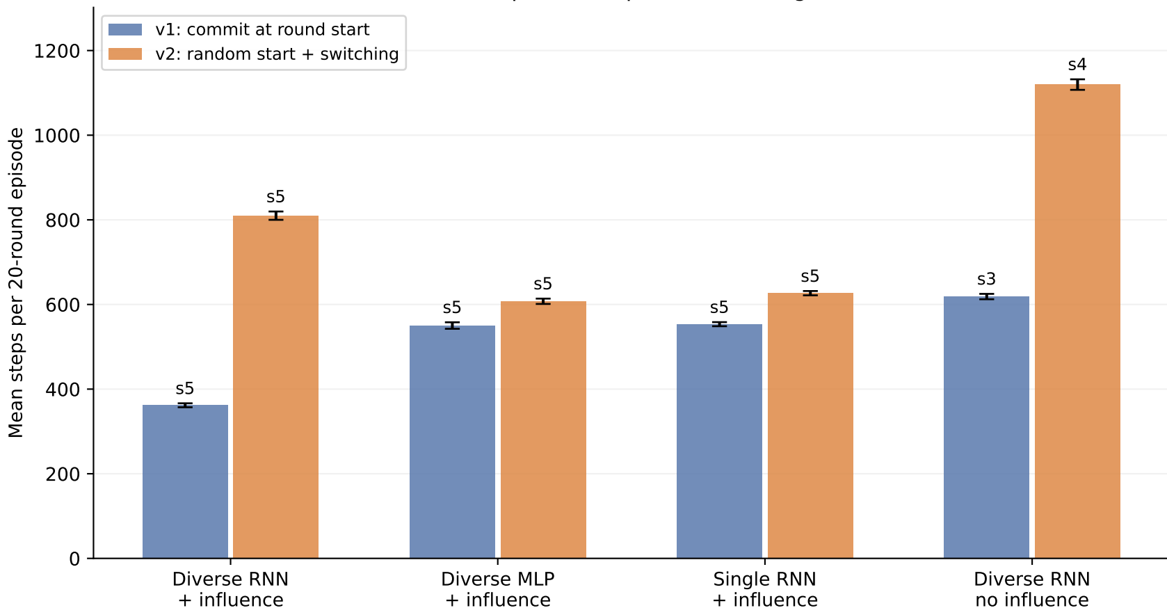
Held-out episode steps: best training seed
