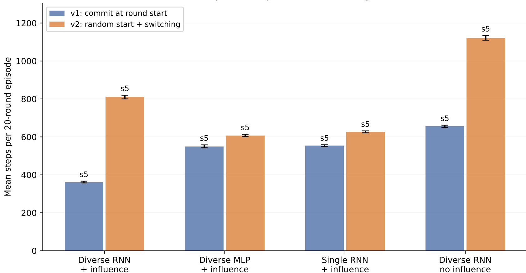
Held-out episode steps: common training seed 5
