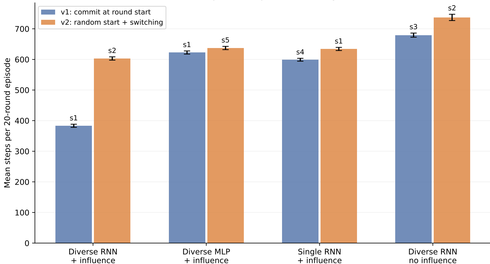
Held-out episode steps: best training seed
