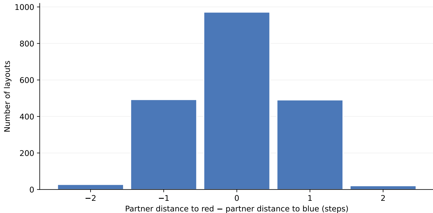
Partner distance difference across all 2,000 layouts Mean -0.01 · median 0
