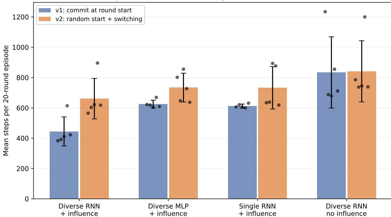
Steps taken with held-out partners: v1 versus v2
