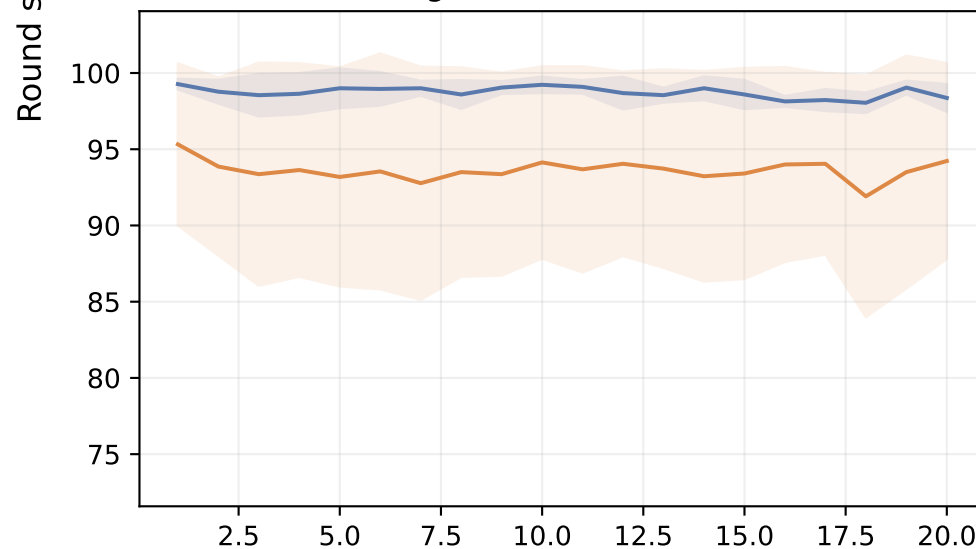
Single RNN + influence
