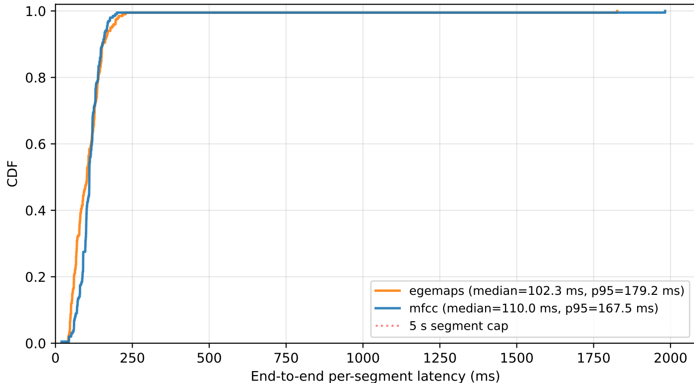
Per-segment latency CDF (S24 Ultra, TorchScript)
