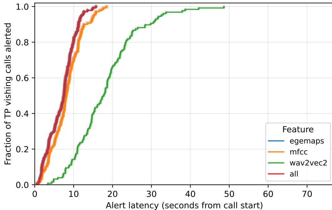
EMA (best \alpha , \tau on val)
