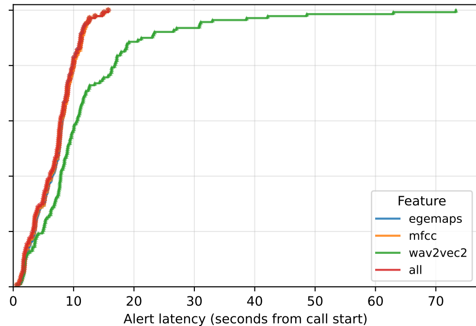
Running-max (best \tau on val)
