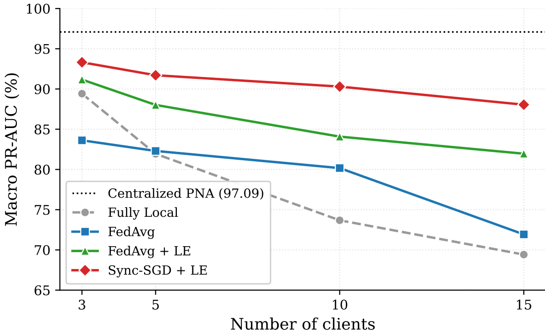
Macro PR-AUC vs. Number of Clients (METIS split)
