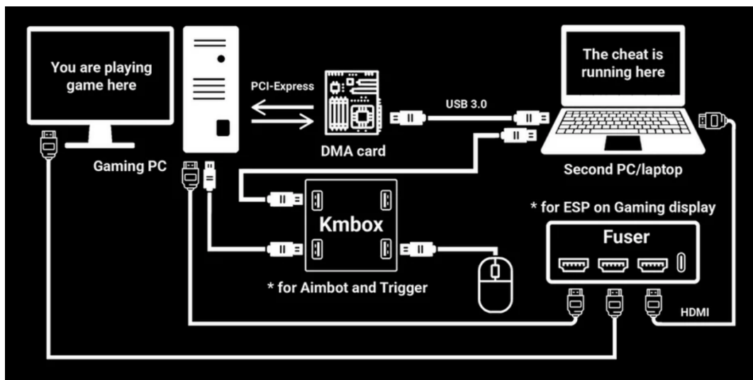
Figure 5: Infrastructure of a DMA cheat setup
