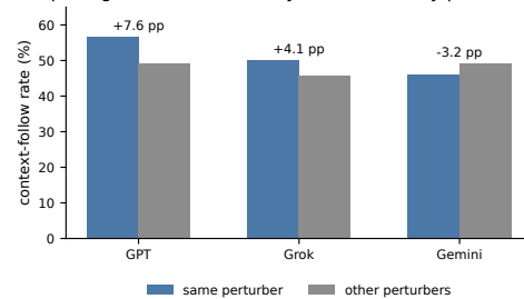
Figure 6: Generator-side self-affinity, retained as descriptive only. Same-perturber context-follow rates are confounded by provider-specific perturbation type preferences.
