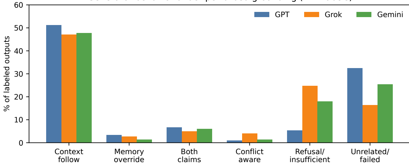
Generator behavior under perturbed grounding (LLM labels)
