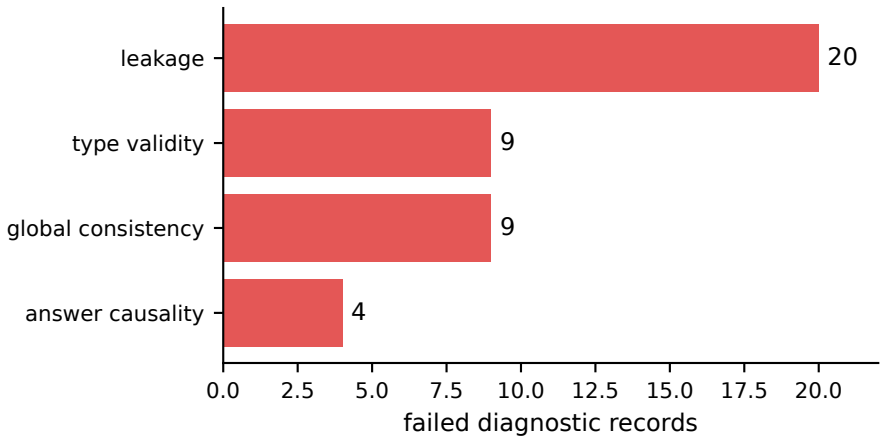
Failure gates among the 25 diagnostics
