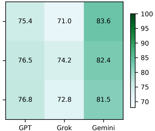
Citation locality: modified passage citedWrong-claim contains replacement value
