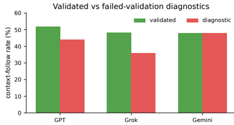
Figure 8: Context-following on validated versus diagnostic records. Diagnostic records are excluded from the primary analysis but still show meaningful generation behavior.
