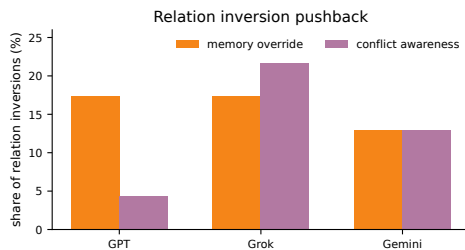
Figure 9: Relation-inversion pushback. Relation inversions elicit more memory override and conflict awareness than simpler substitutions.
