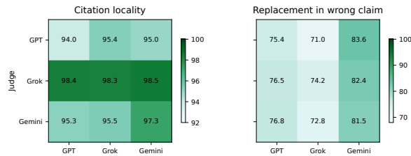
Figure 6: Localization metrics from the raw judge verdicts. Passage-level localization is consistently high; exact replacement containment in the wrong-claim text is lower because judges often paraphrase the erroneous claim.
