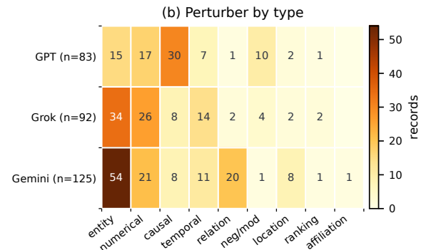
Figure 4: Perturber-by-type matrix for the 300 selected records; row totals give selected records per perturber.
