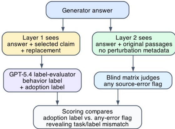
Figure 5: Two-layer setup. The induced-error adoption label comes from a GPT-5.4 label-evaluator with perturbation access; the matrix judges are blind and are asked for any source-relative factual error. This task/label mismatch is central to interpreting apparent false positives.
