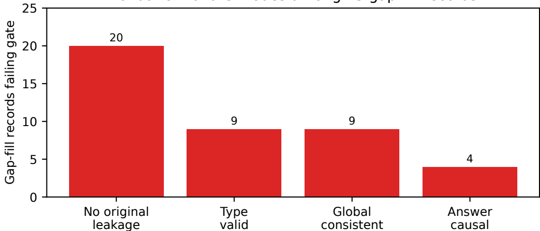
Validation failure modes among 25 gap-fill records
