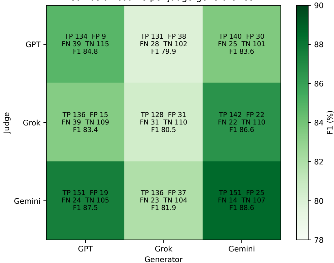
Confusion counts per judge-generator cell
