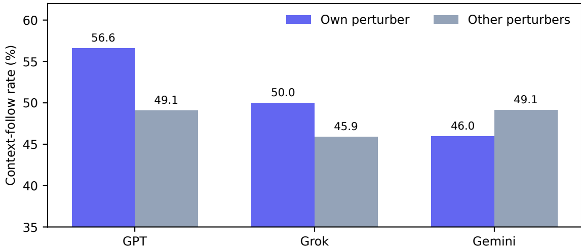
Generator-side self-affinity
