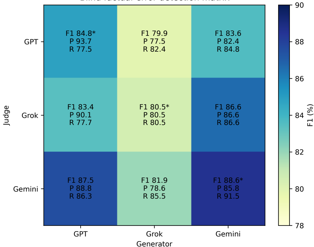
Blind factual-error detection matrix
