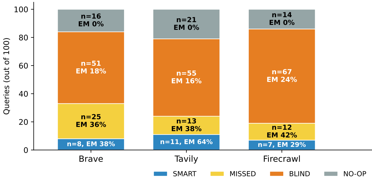
Smart / Missed / Blind / No-op partition with EM%
