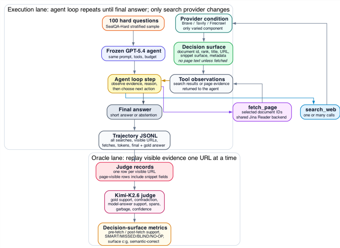
Figure 1: Execution and judging pipeline. The provider returns only the pre-fetch decision surface: ranked URLs, snippets, and metadata. The agent may issue multiple search_web or fetch_page calls in one turn. Every visible URL is replayed to the Kimi judge in the same representation the answer model saw, yielding per-URL oracle labels.
