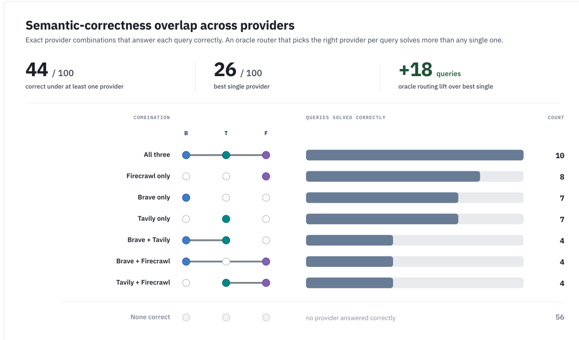
Figure 4: UpSet-style semantic-correctness overlap across providers. Rows show exact provider combinations that answer each query correctly; an oracle provider router would solve 44 queries, above the best single provider.
