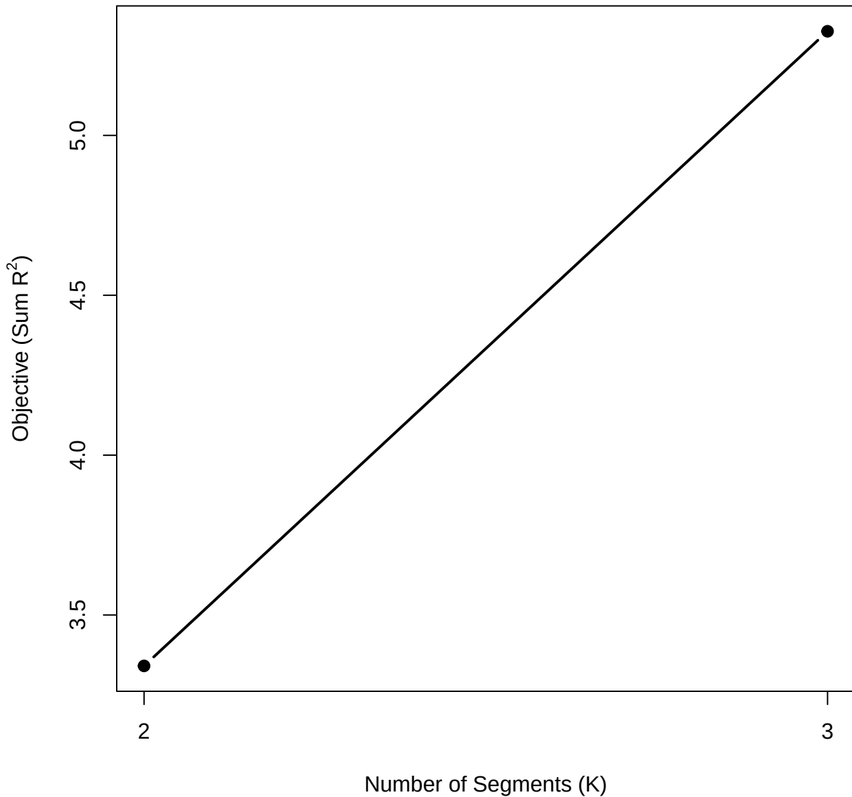
PLS-POS: Objective Criterion vs K
