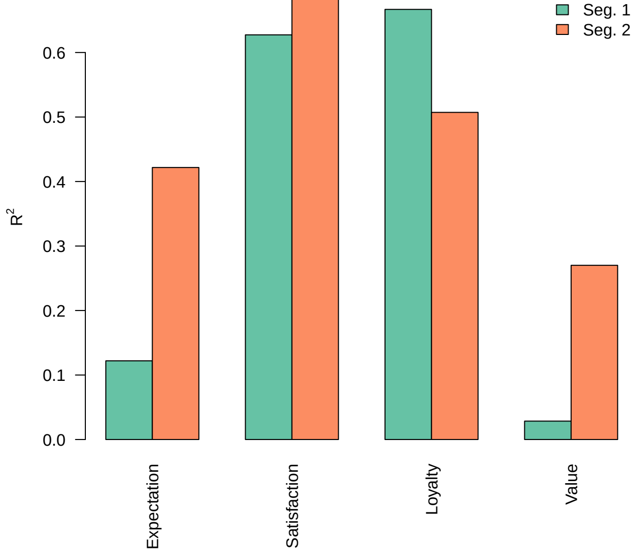
PLS-POS: R 2 per Construct (K = 2 )
