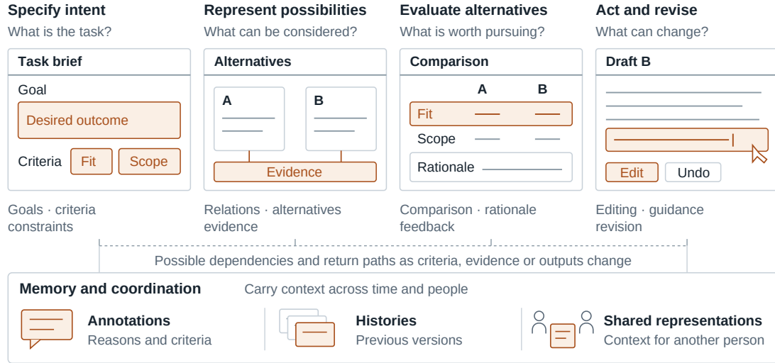
Fig. 12. From task intent to action. Four overlapping functions offer an activity-oriented view of the mechanism taxonomy. Memory and coordination connect them across time and people. The sketches show criteria, alternatives, comparison, and revision; the shared strip keeps decisions and their context available across these activities. The accompanying source examples illustrate these relationships [43, 73, 120, 137].
