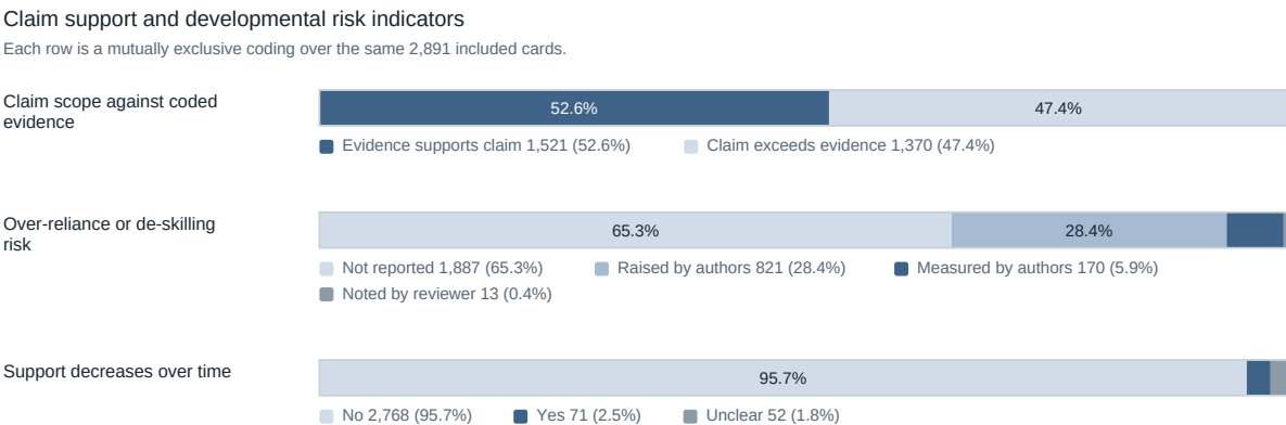
Figure 51: Claim scope exceeds coded evidence in nearly half of included cards, over-reliance is raised far more often than it is measured, and decreasing support is rare. Each row is a mutually exclusive coding over the same 2,891 included cards, and every segment prints its own count and share. A claim-evidence gap records the distance between a card’s stated claim and its linked evidence; it is not an assessment of the underlying paper. Examples, one or two cards per value: claim within evidence: InstructPipe [148].
