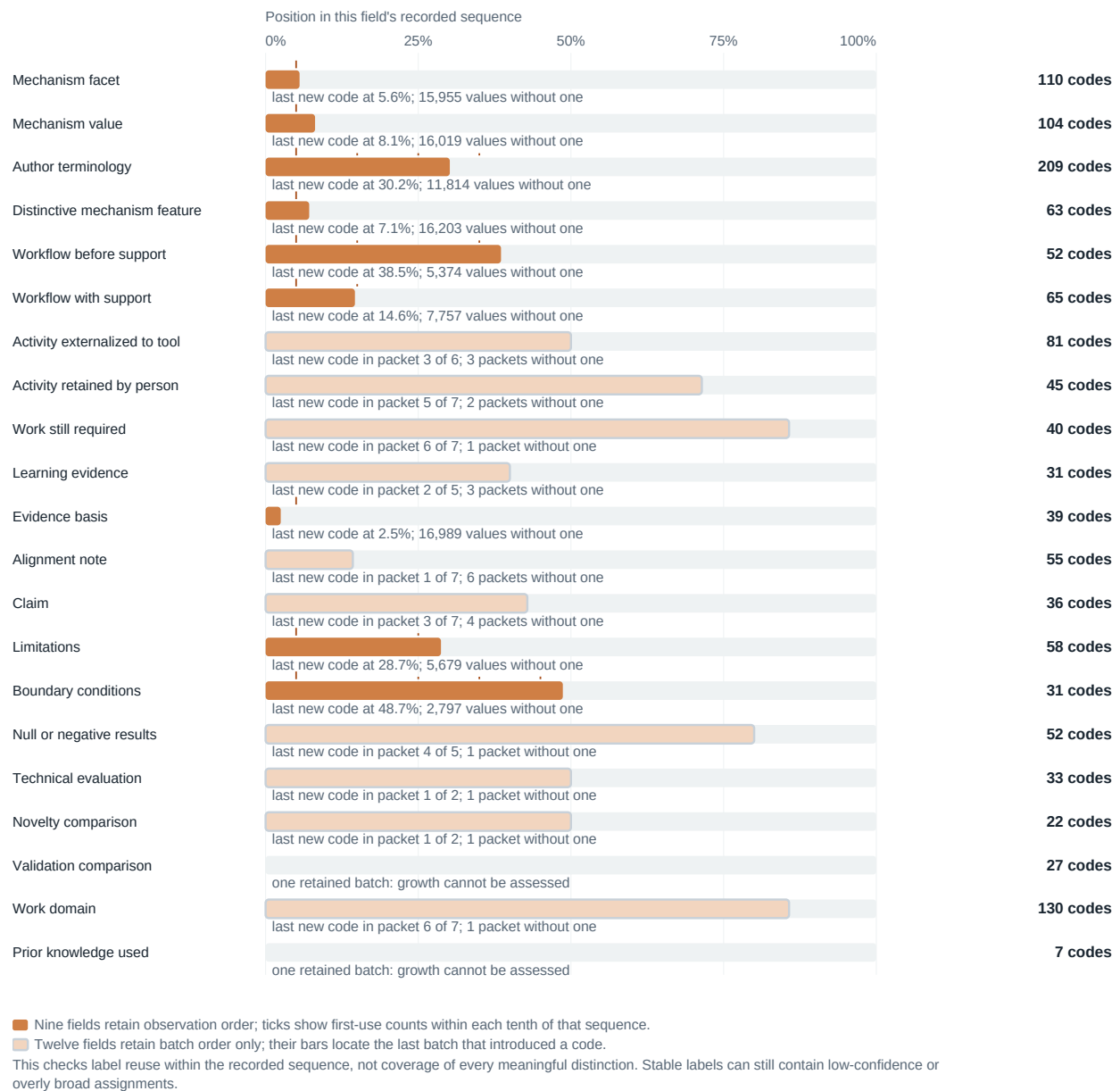
Figure 62: New-code creation within each field of the first coding. Bars locate the last new code in the recorded coding sequence; ticks show new codes by tenth of the sequence. Where only batch order survives, the figure reports batch resolution.
