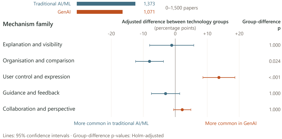
Fig. 10. Between-technology differences in mechanism families among 2,444 papers with usable family coding and classified technology, 2019–2025. Dots show GenAI minus traditional AI/ML prevalence, adjusted for year and venue; lines show pointwise 95% confidence intervals. The p -values test these group differences, with Holm correction across 51 contrasts, rather than change over time. User control retains support in the 2023–2025 and partial-2026 sensitivity windows. Of 3,385 family-coded papers, 540 lack classified technology and 401 classified papers fall outside 2019–2025.
