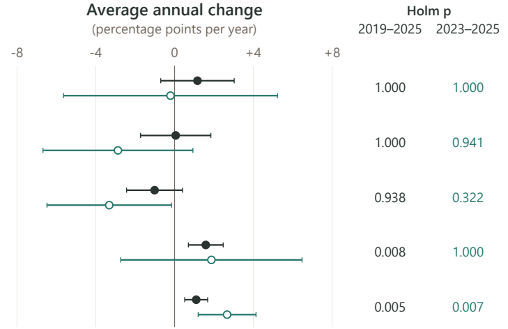
Fig. 11. Average annual change in coded mechanism-family prevalence: 2019–2025 (2,444 papers) and the 2023–2025 sensitivity (1,390). Dots show percentage points per year; lines show pointwise 95% venue-clustered confidence intervals. The technology mix is held fixed at 43.75% GenAI in both windows. Positive values indicate increasing prevalence. These are temporal slopes, not the overall technology-group differences in Figure 10. Appendix D.3 gives the methods, changing-gap estimates and all ten tests used for Holm correction within each window.
