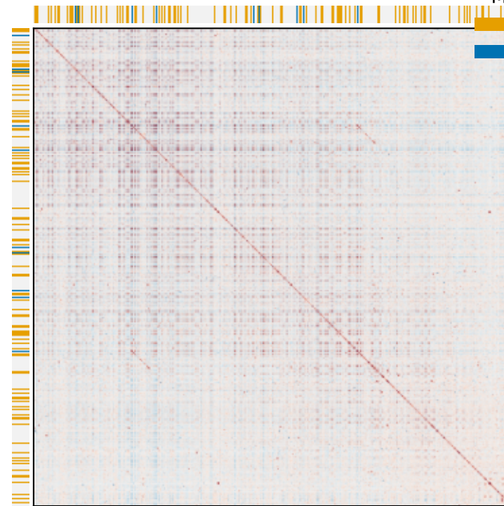
m5_chr7_120066194_120070289
