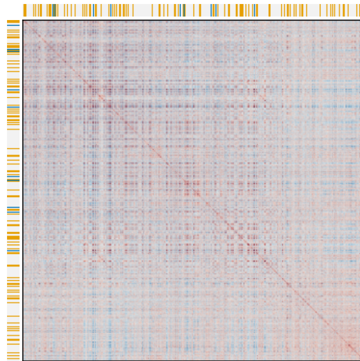
m4_chr7_120066194_120070289
