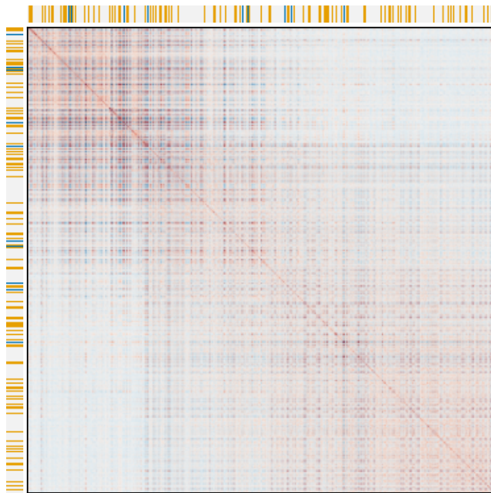
m0_chr7_120066194_120070289
