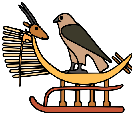
Figure 1: Hieroglyph G10
