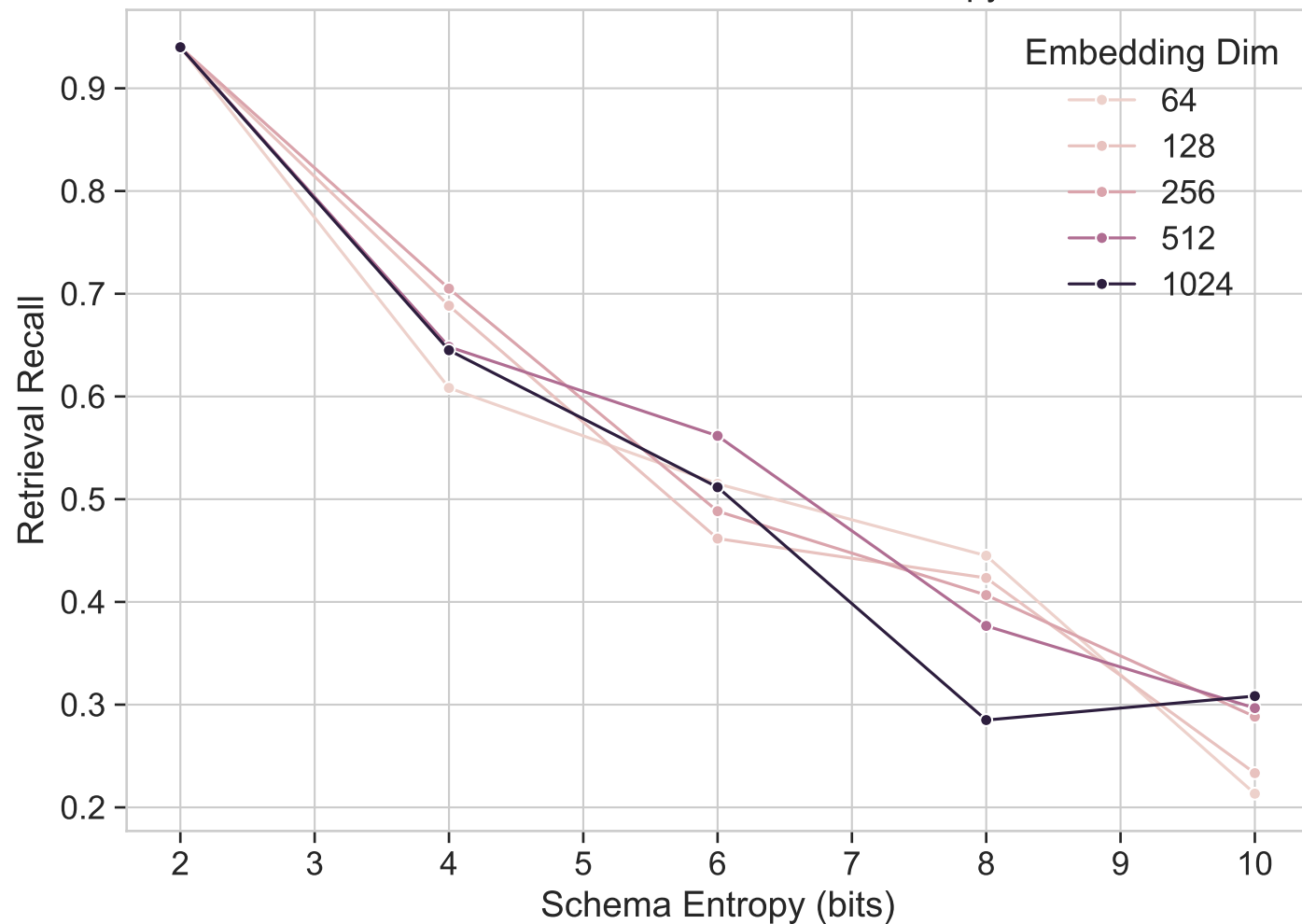
Retrieval Recall vs Schema Entropy
