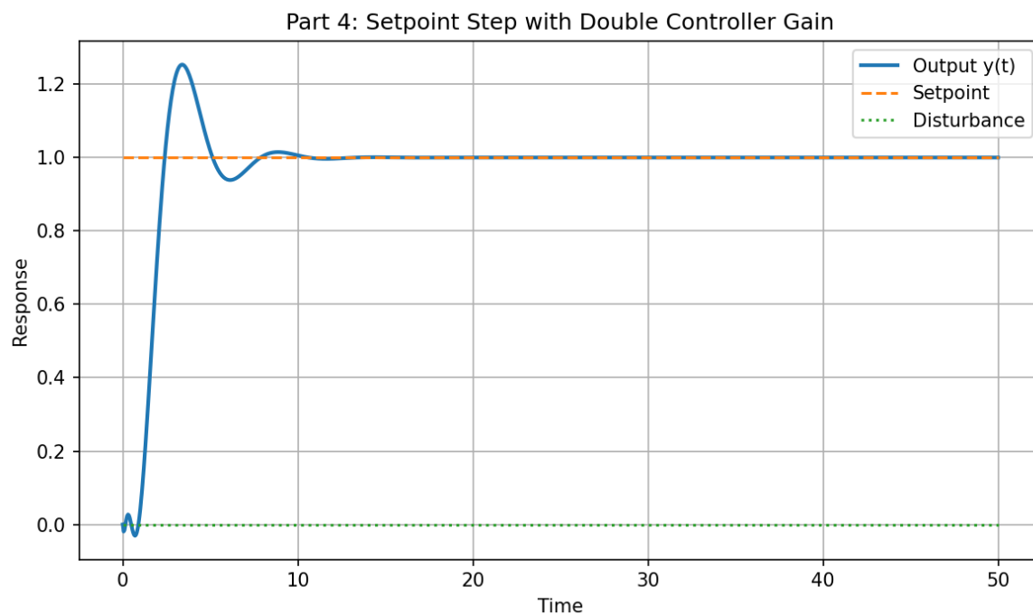
Figure 3: Closed-loop response to a unit step in setpoint with doubled controller gain.
