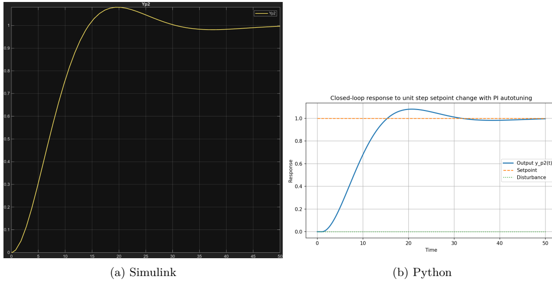
Figure 5: Closed-loop response to step change in setpoint and no step disturbance with PI autotuning.
