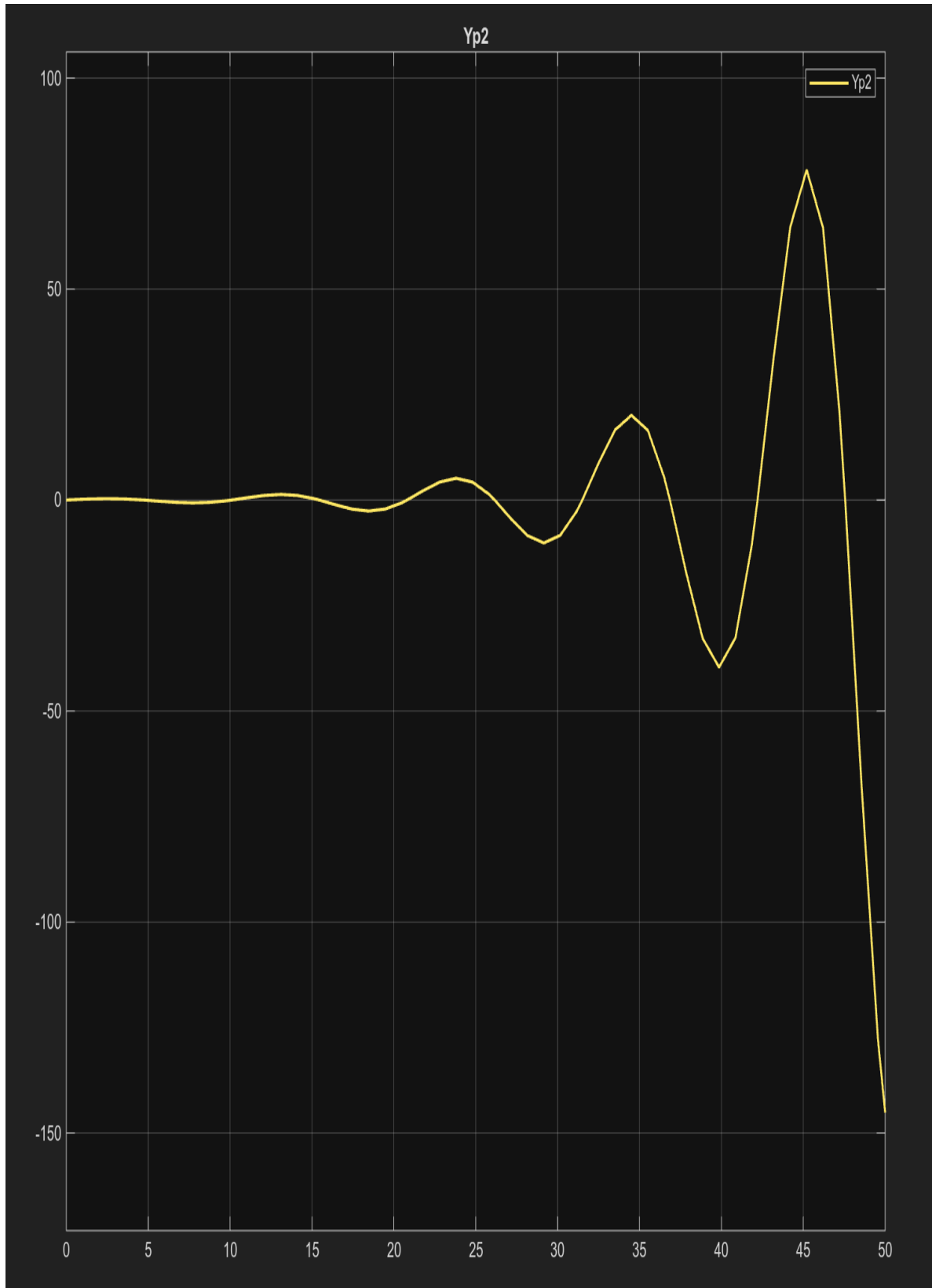
Figure 2: Closed-loop response to no step change in setpoint and a unit step change in disturbance from Simulink.
