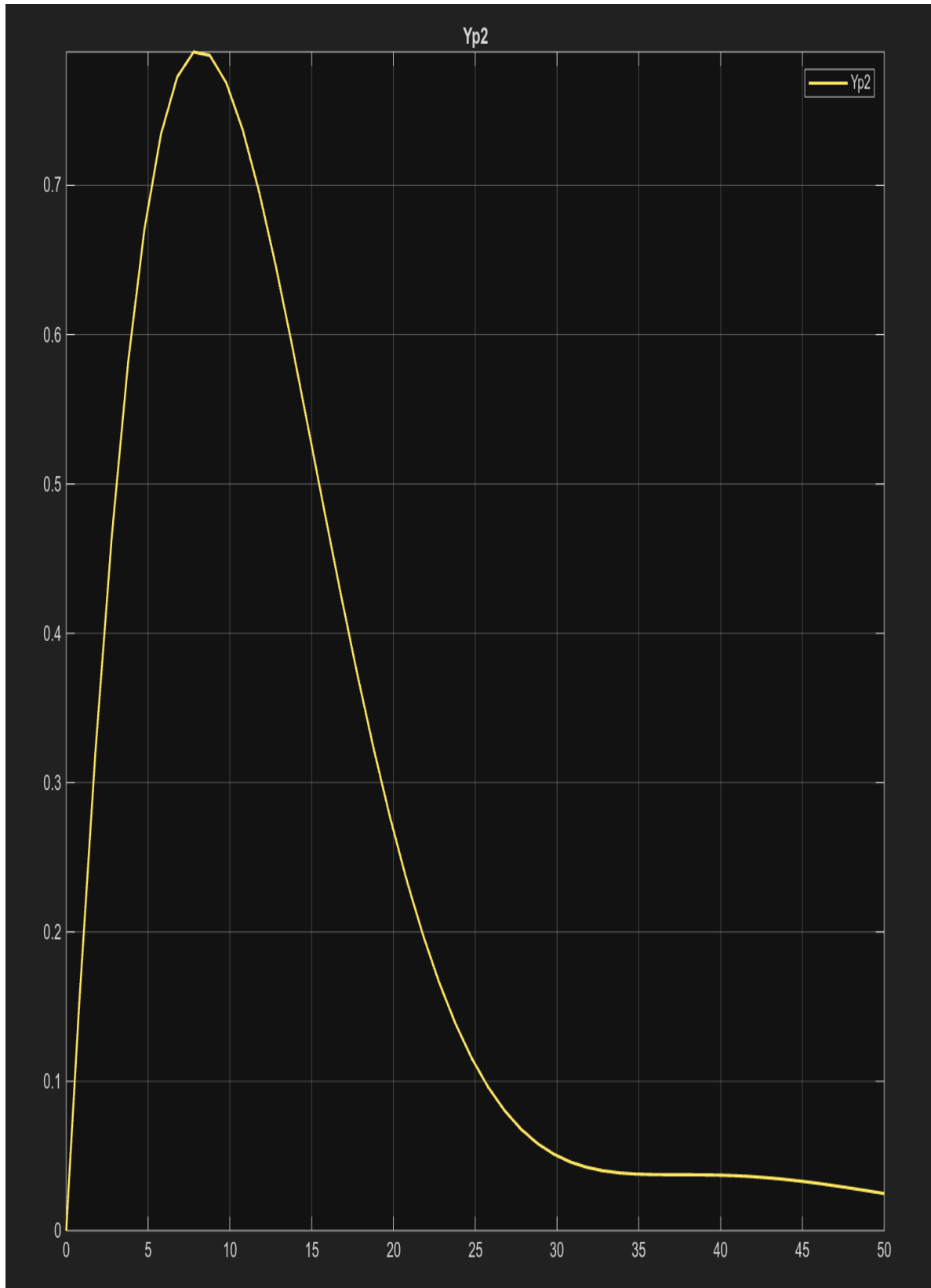
Figure 5: Closed-loop response to no step change in setpoint and a unit step disturbance using PI autotuning from Simulink.
