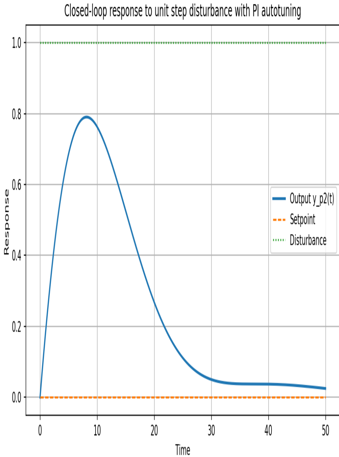
Figure 4: Closed-loop response to no step change in setpoint and a unit step disturbance using the Simulink autotuned PI values in Python.
