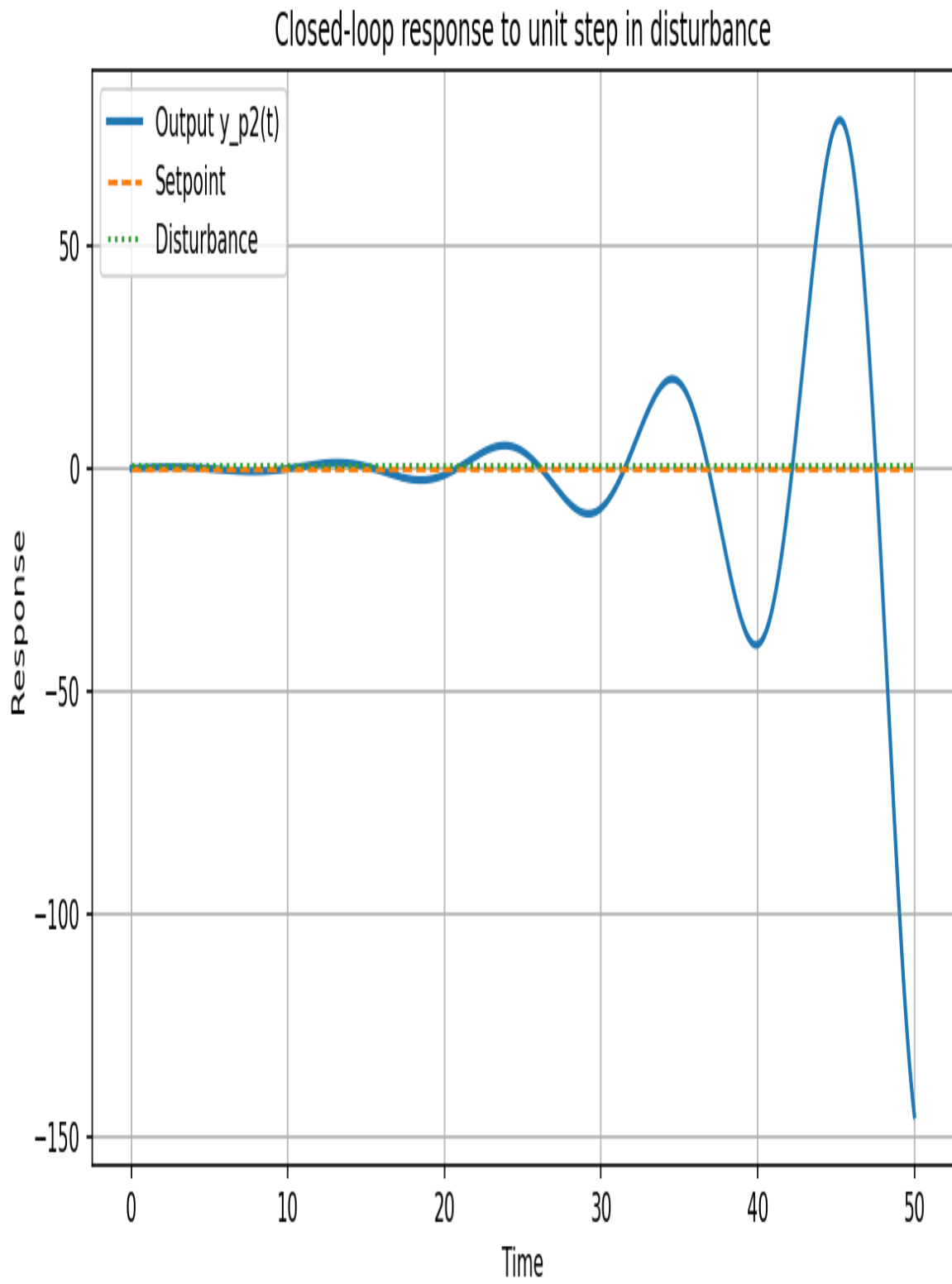
Figure 3: Closed-loop response to no step change in setpoint and a unit step change in disturbance from Python.
