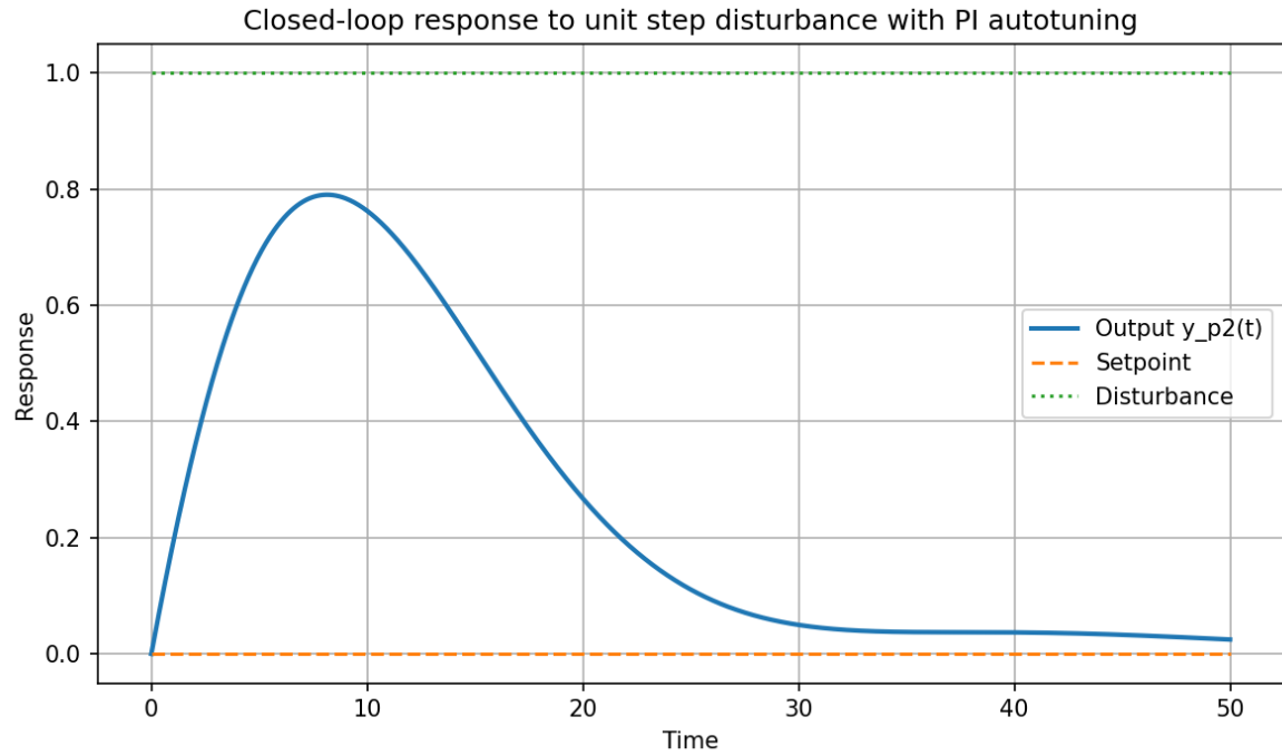
Figure 4: Closed-loop response to no step change in setpoint and a unit step disturbance using the Simulink autotuned PI values in Python.
