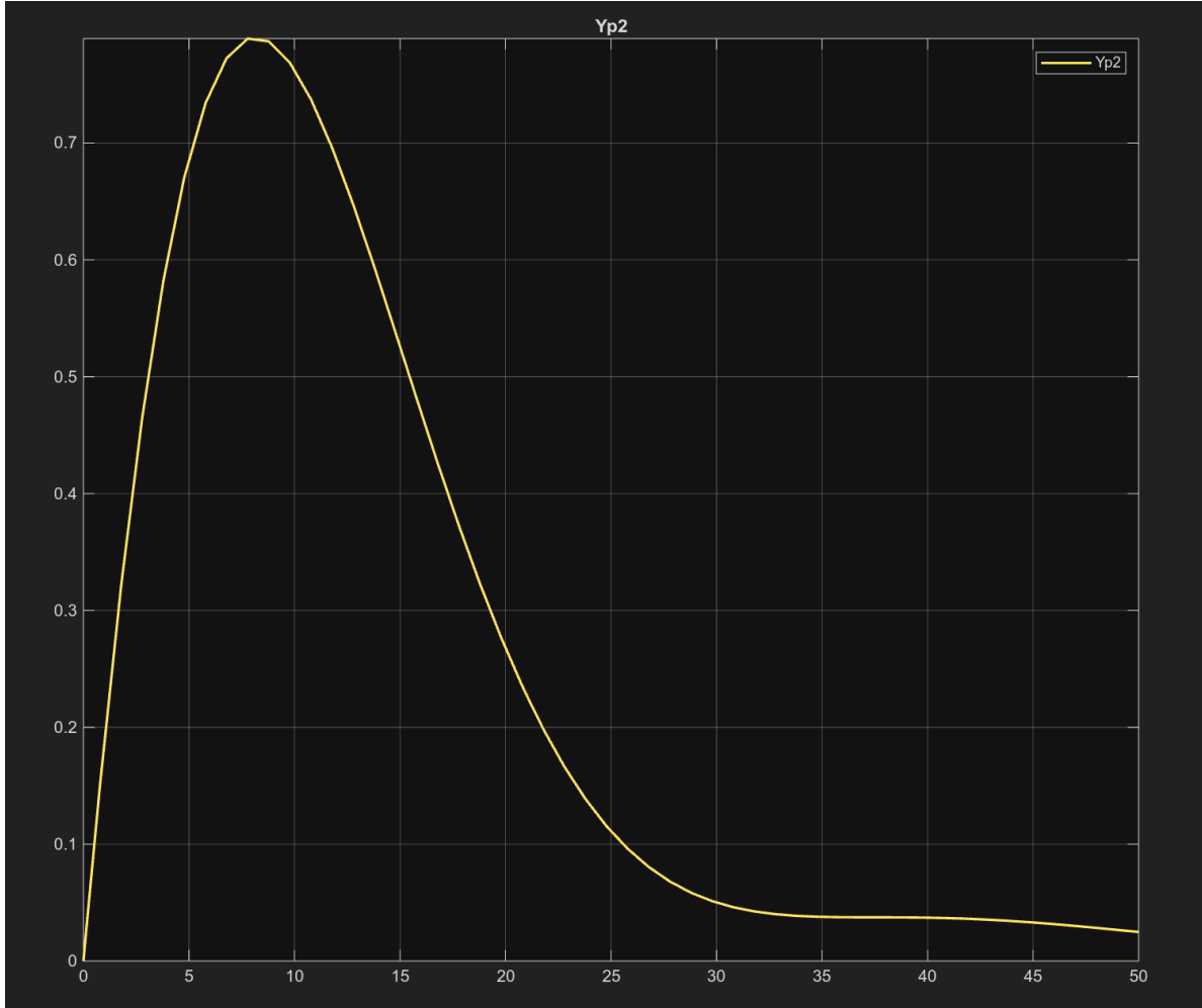
Figure 5: Closed-loop response to no step change in setpoint and a unit step disturbance using PI autotuning from Simulink.
