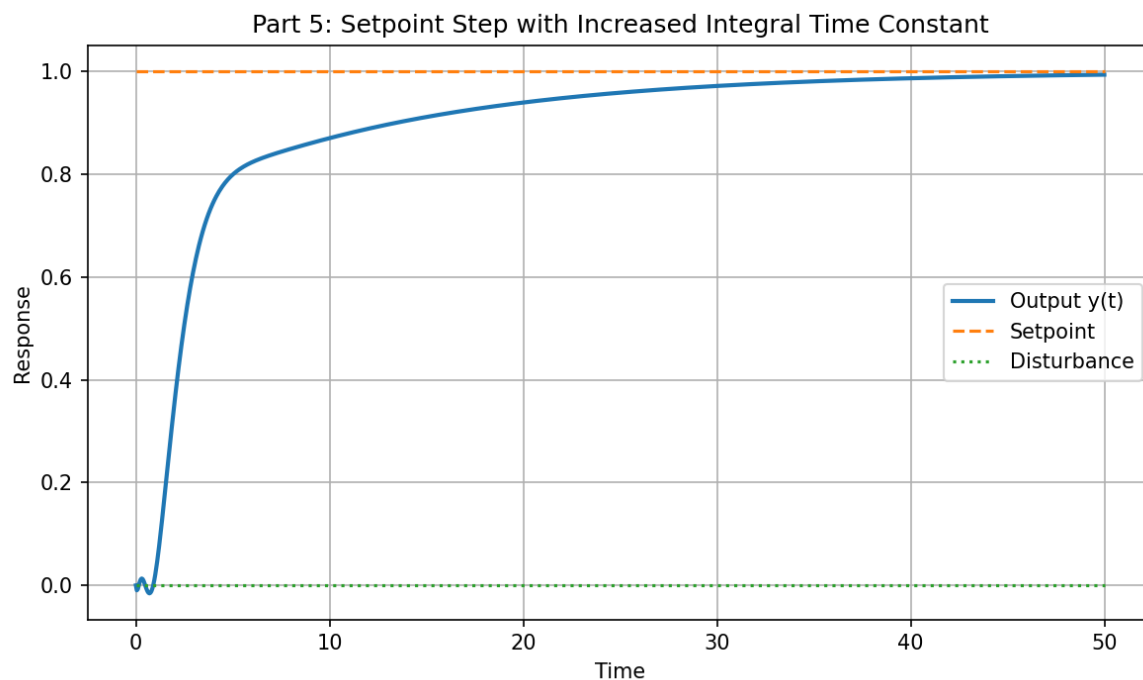
Figure 9: Closed-loop response to a unit step in setpoint with increased integral time constant.
