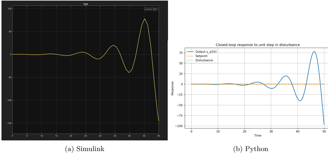
Figure 3: Closed-loop response to no step change in setpoint and a unit step change in disturbance with no cascade control and no autotuning.
