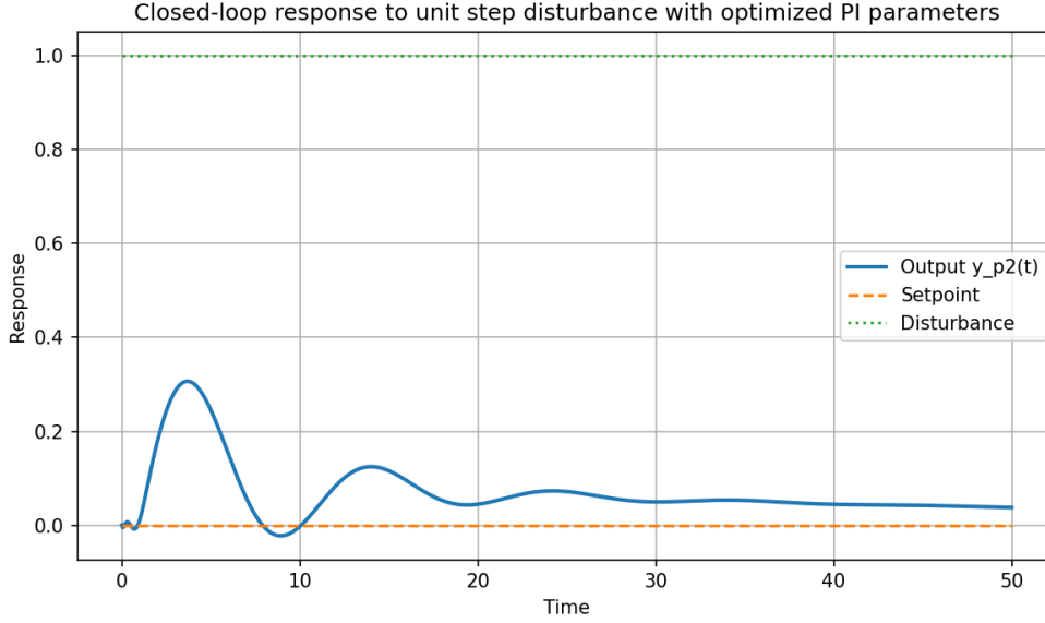
Figure 2: Closed-loop response to unit step disturbance with optimized PI parameters.
