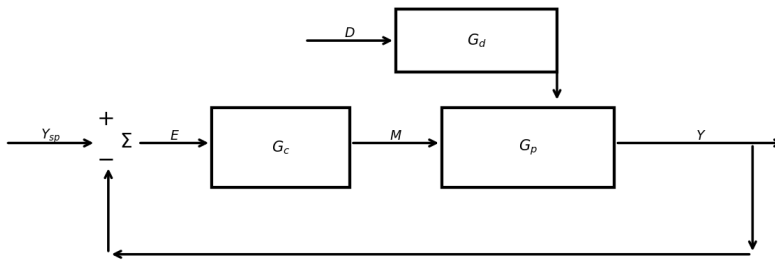
Basic feedback control with input-side disturbance
