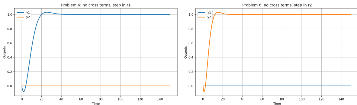
(a) Step in r_1
