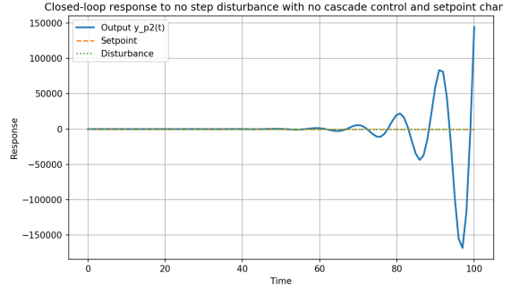
(b) Python
