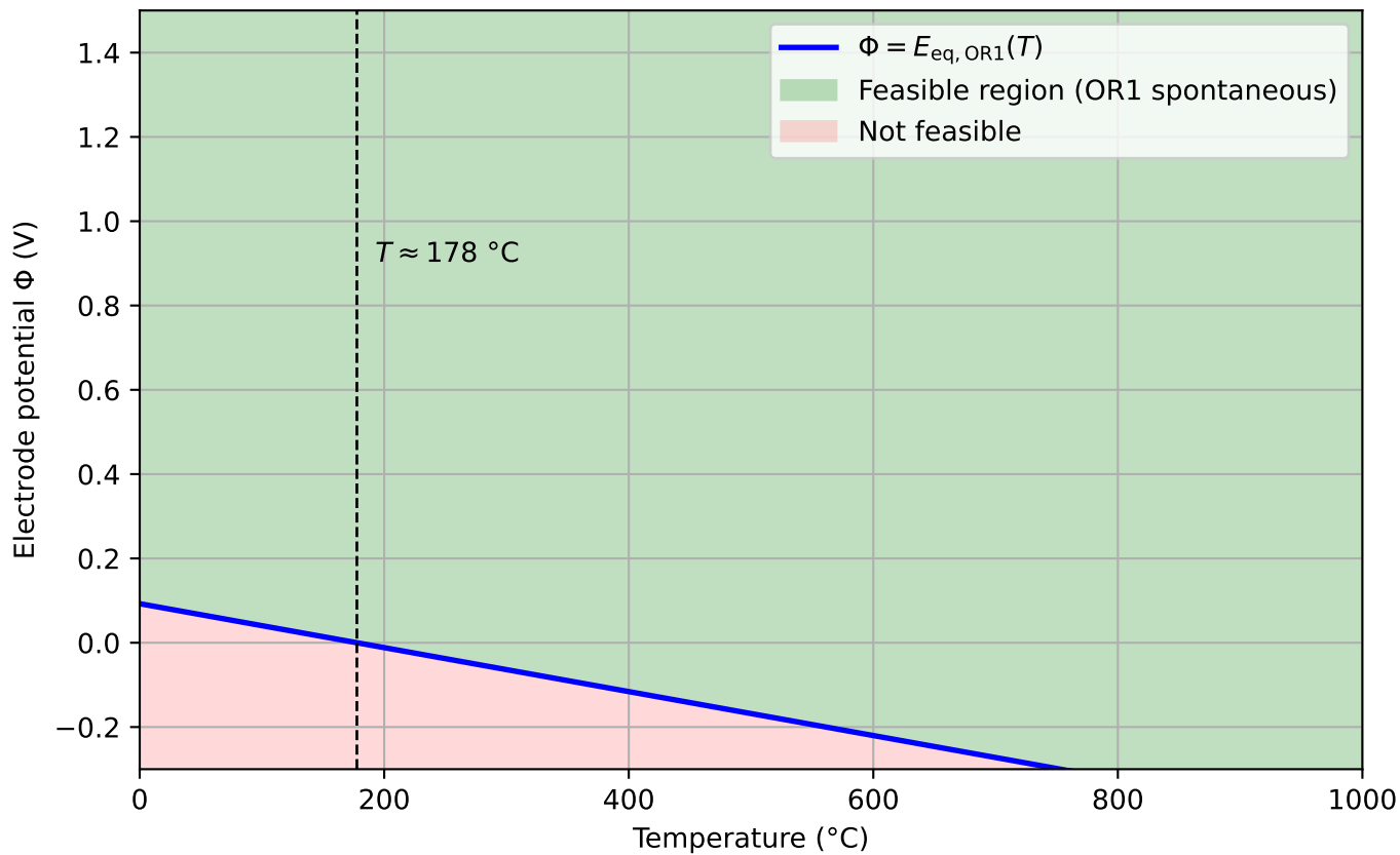
Feasibility map for OR1: \text{CH}_3\text{OH} \rightleftharpoons \text{CO} + 4\text{H}^+ + 4\text{e}^-
