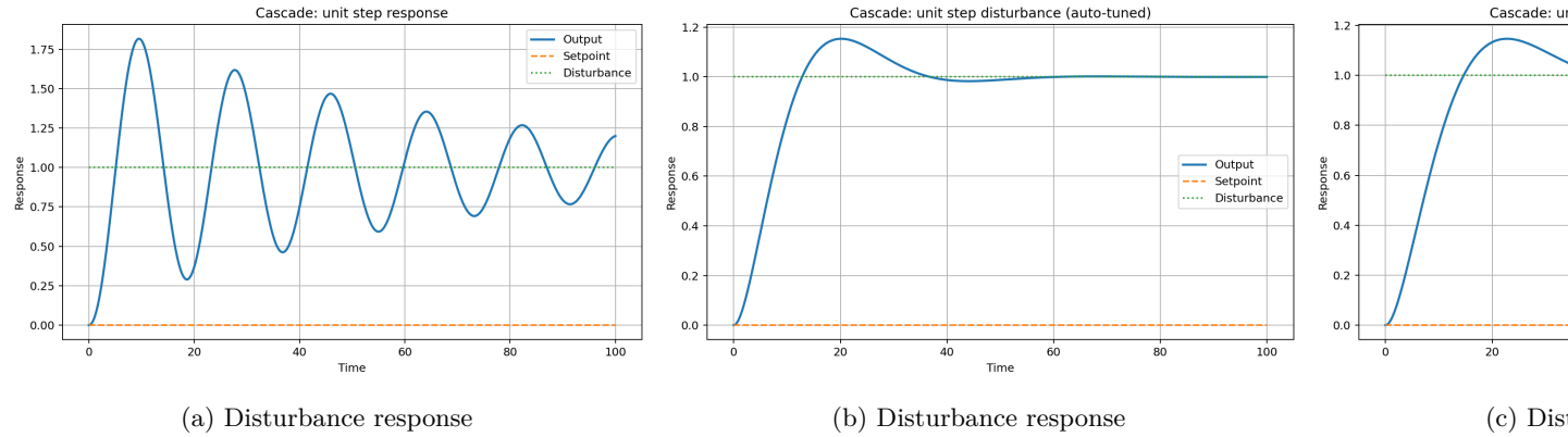
Figure 4: Problem 2 responses with cascade control and unit step disturbance.
