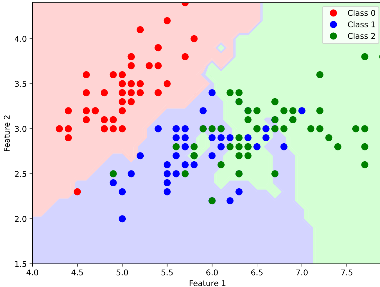
K-NN Decision Boundary (k=5)
