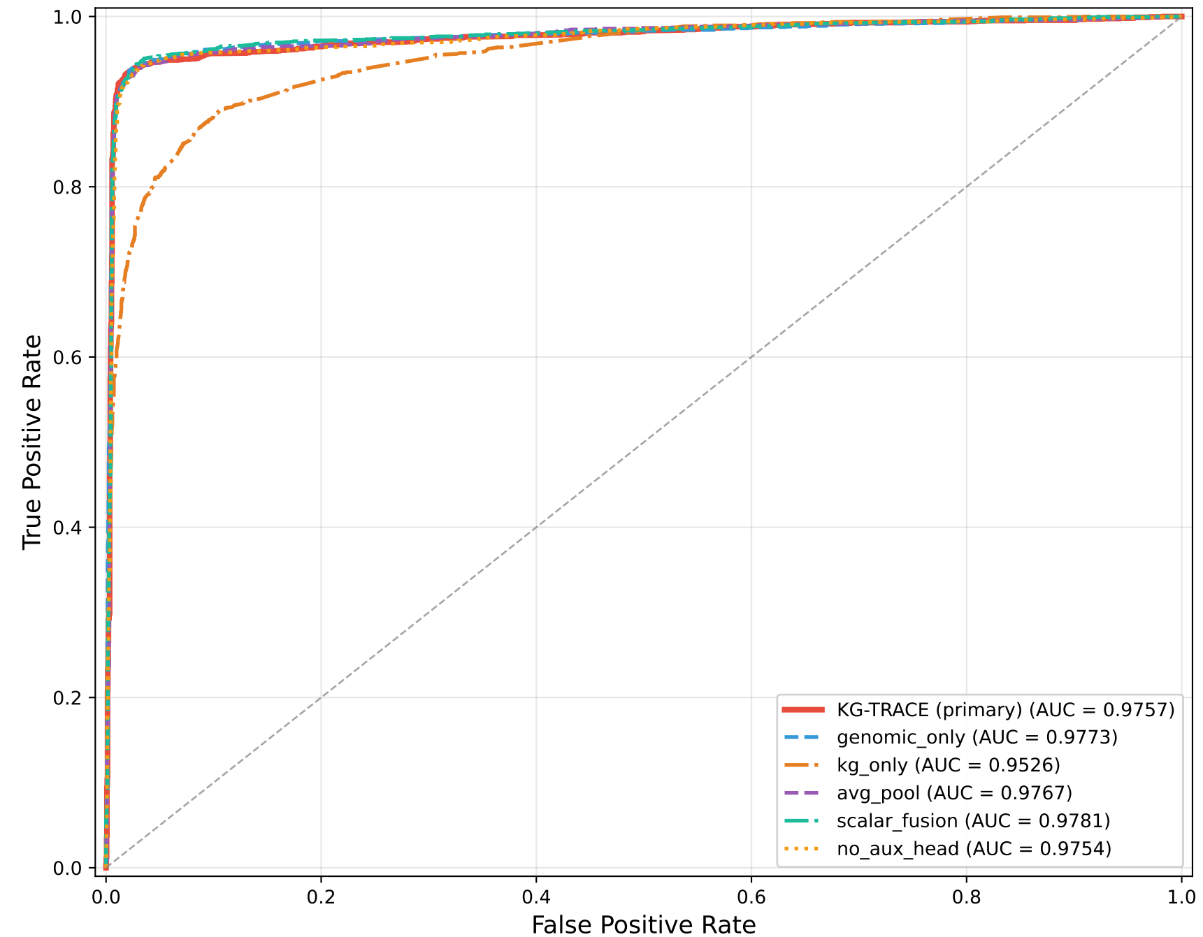
B) ROC Curves — Ablation Study
