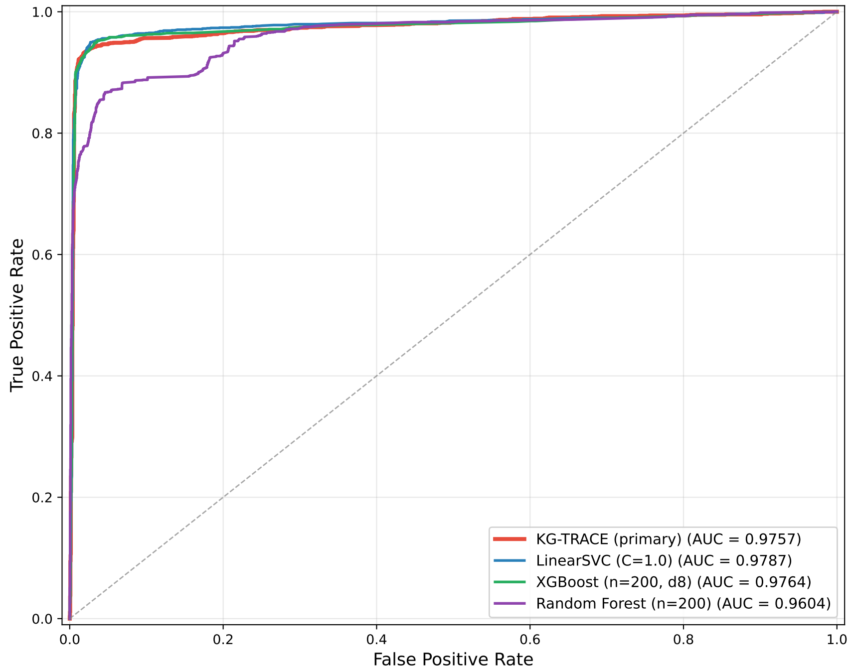
A) ROC Curves — Baselines
