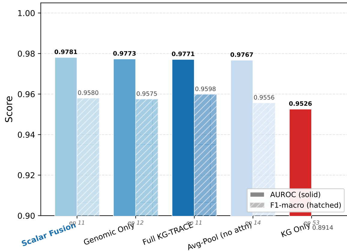
(B) Ablation Study — AUROC & F1-macro (100-epoch runs, early stopping; epoch at convergence shown)
