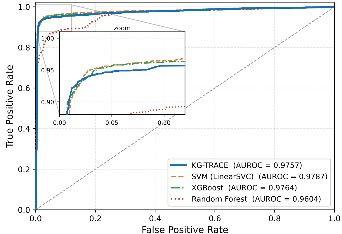
(A) ROC Curves — KG-TRACE vs Baselines n_{\text{test}} = 5,665 (INH, M. tuberculosis )
