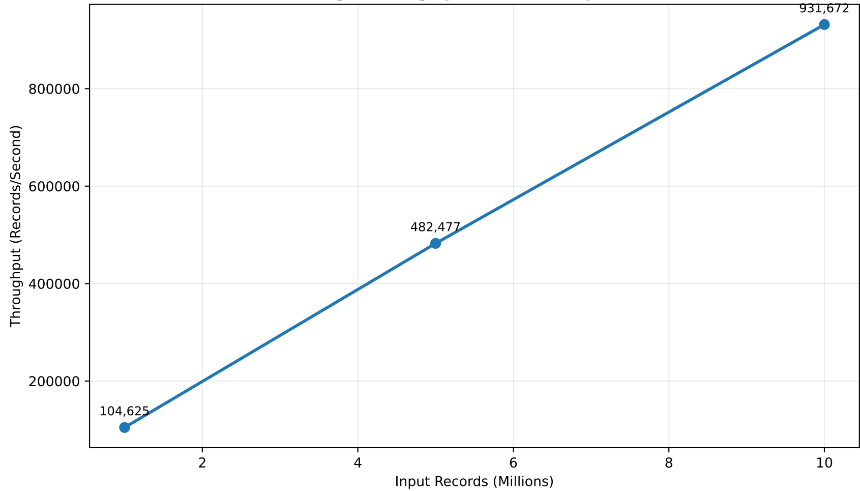
Processing Throughput Across Input Volumes
