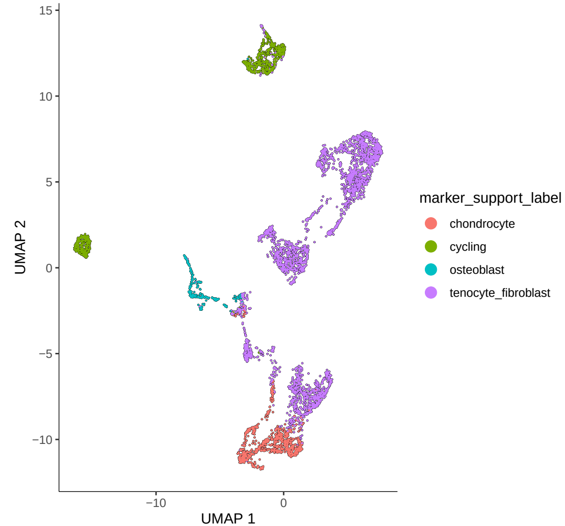
Monocle3 native UMAP
