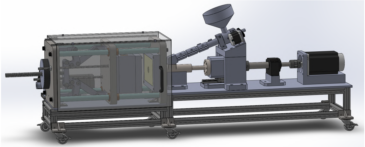
Injection Molder Full CAD
