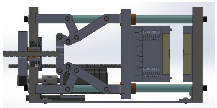
CEM Section View
