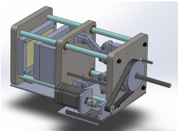
Clamping, Ejection, and Mold (CEM) Units View
