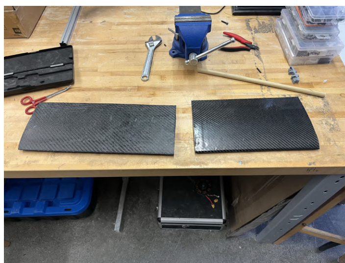
Split Molded Airfoil vs Foam Core Layup
