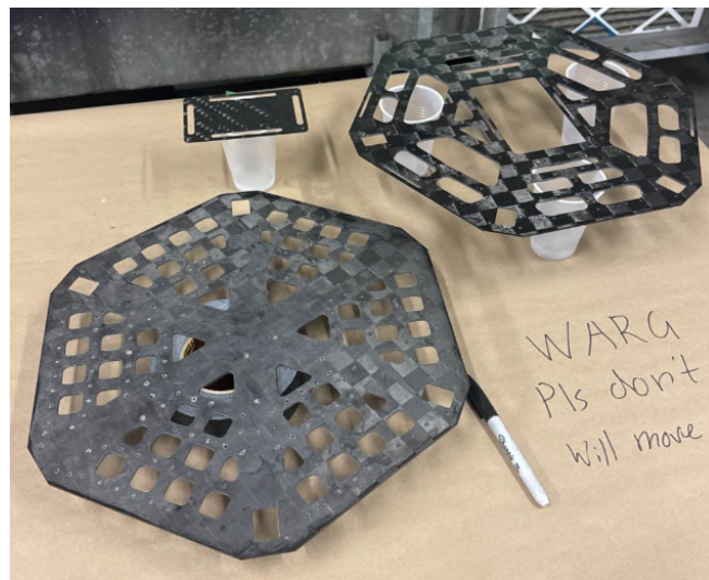
Wet Layup Post-Processed
