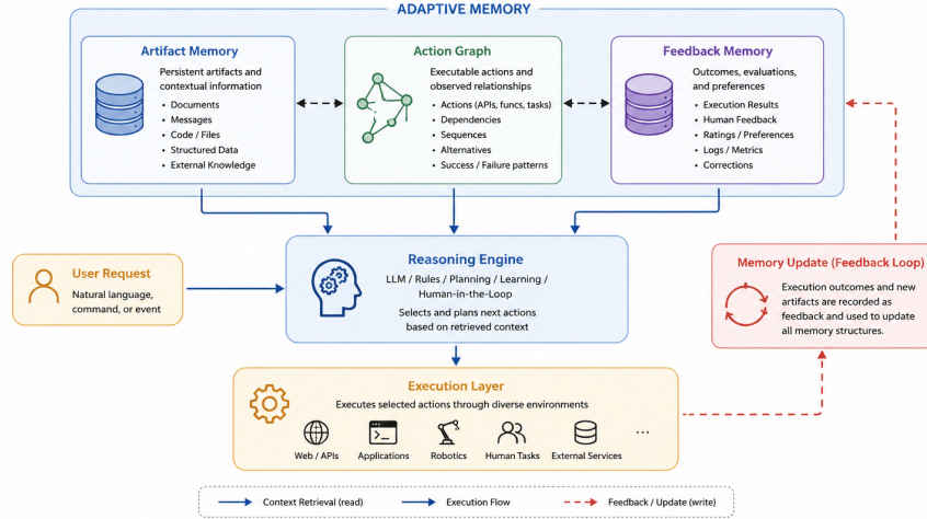
Figure 1: Overview of the Semut Adaptive Architecture and information flow.
