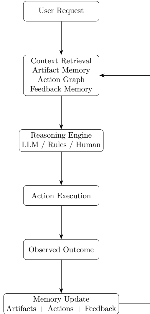
Figure 2: The Semut adaptive feedback loop. Each interaction retrieves context from Artifact Memory, Action Graph, and Feedback Memory, executes selected actions, observes outcomes, and updates all memory structures for future reasoning.
