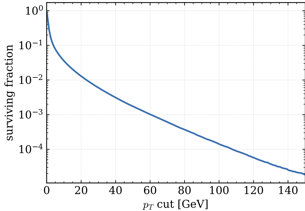
survival fraction vs p_T cut
