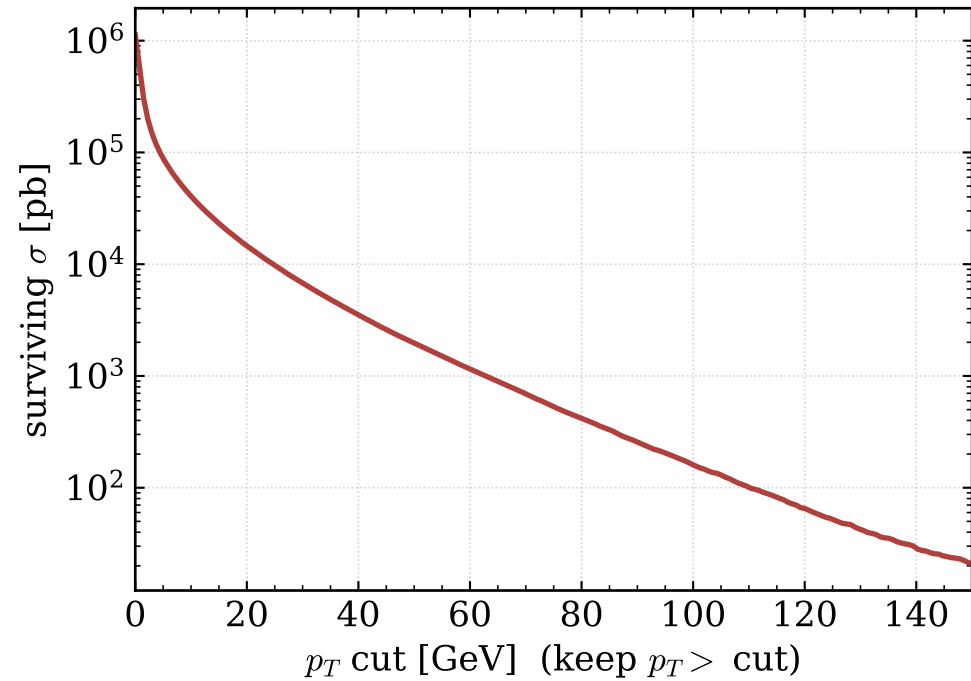
K_L cross section vs p_T cut
