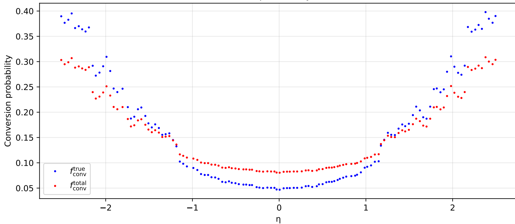
Photon conversion probability — CMS Phase-1
